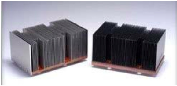
Figure 4.- Typical Image of a Bonded fin Heat Sink [9]
