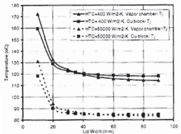
Figure 8: Junction Temperature as a Function of Lid Size for Vapor Chamber and Solid Copper Base for 400 and 50,000 W/m 2 K Heat Transfer Coefficients [1]
